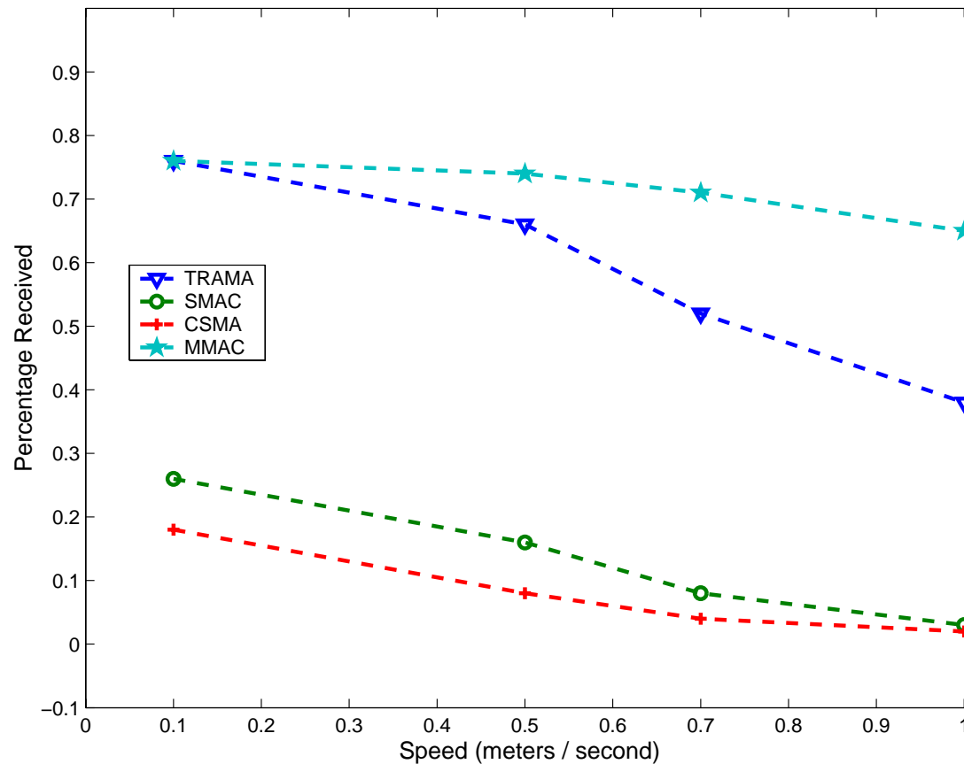
Percentage of Packets Received (increasing Mobility)
