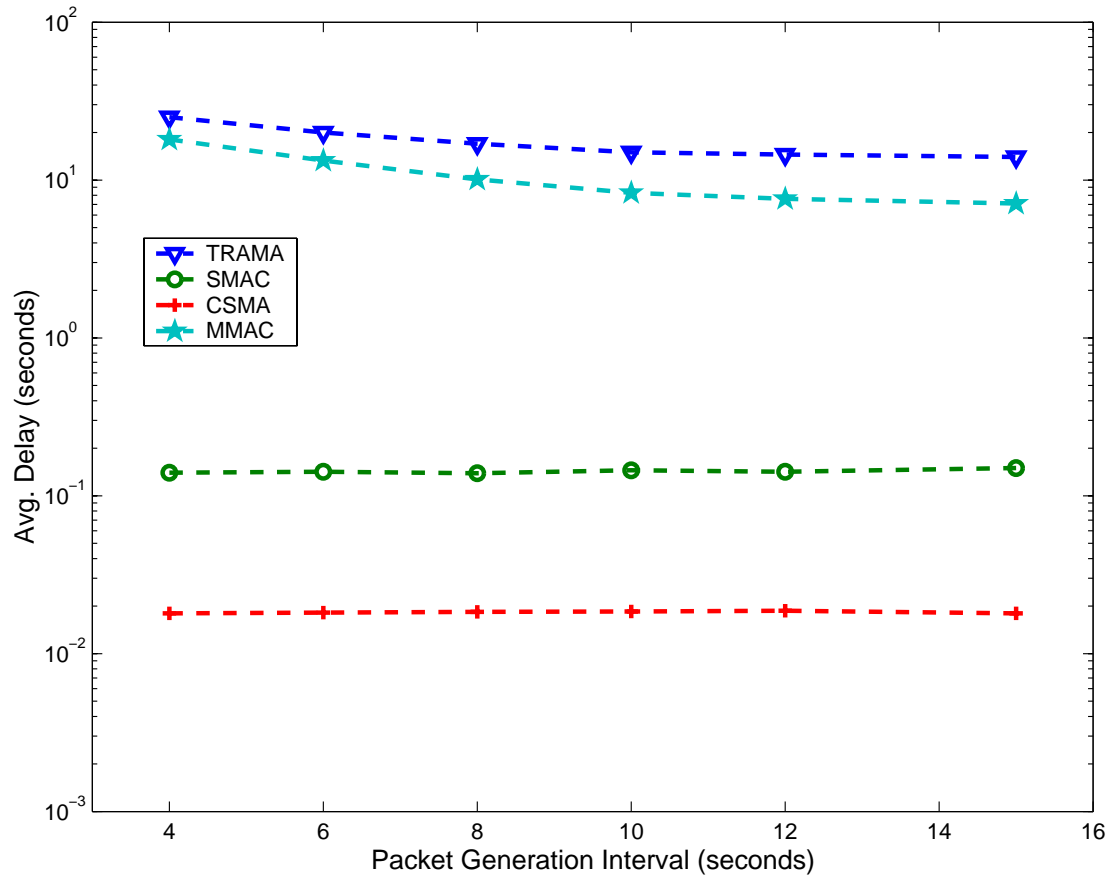
Average Packet Delay (Variable Traffic)
