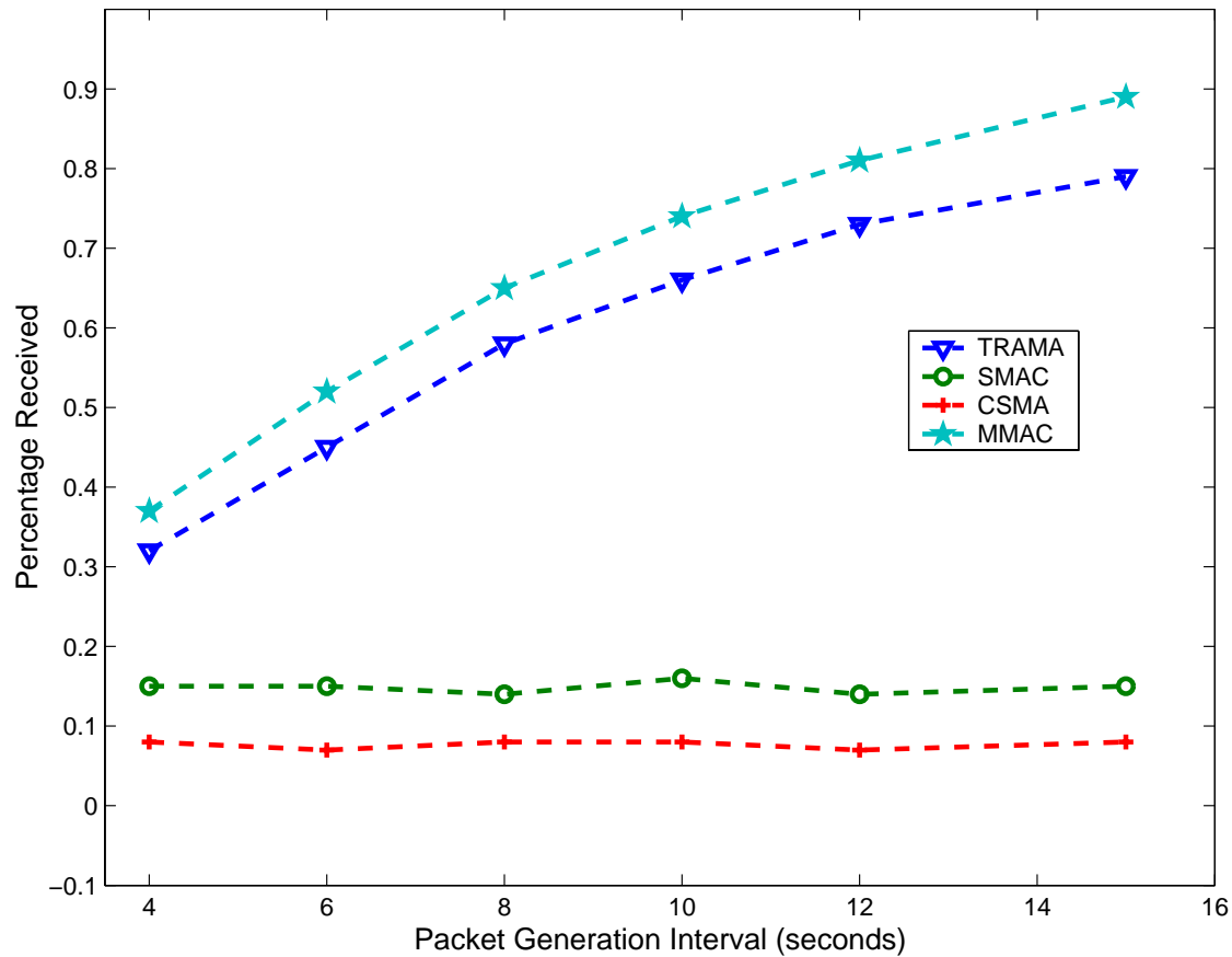
Percentage of Packets Received (Variable Traffic)
