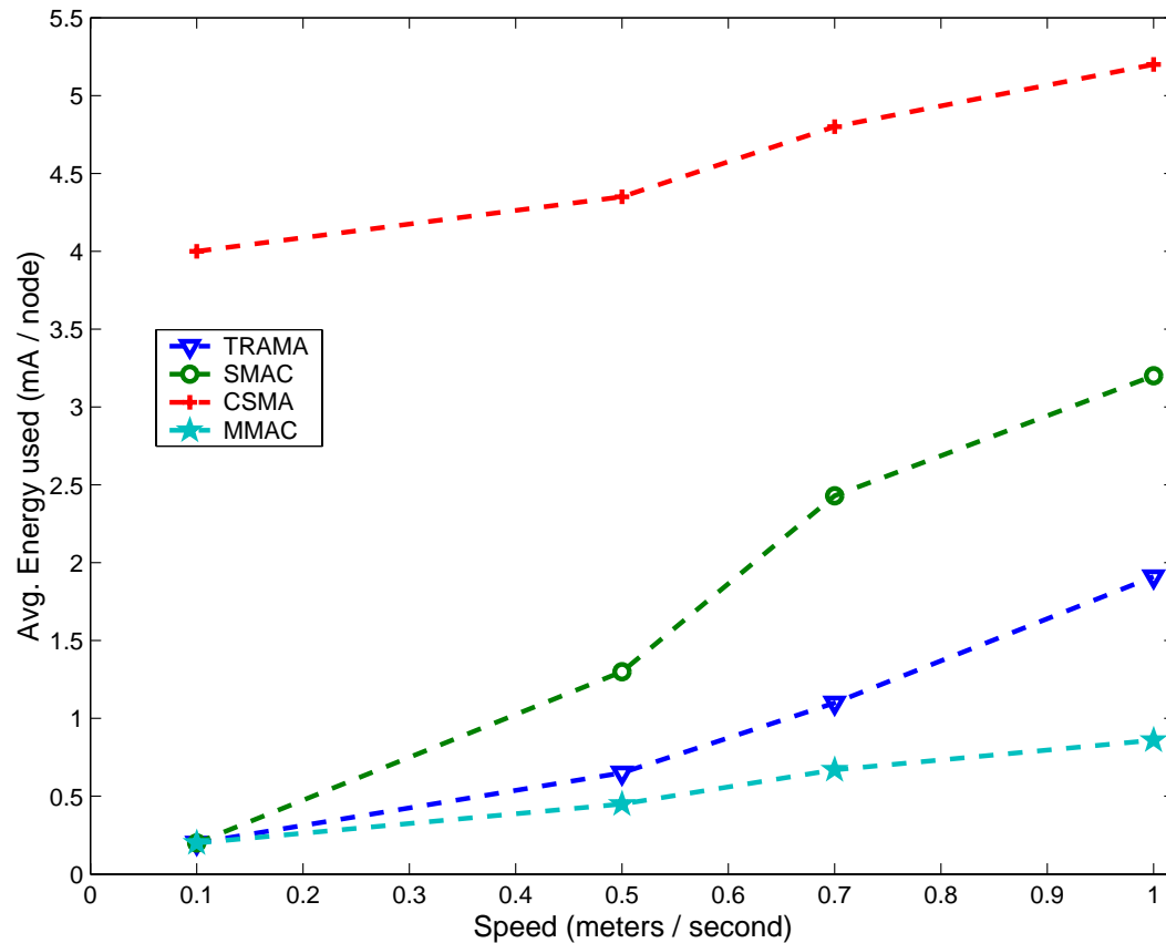
Average Energy consumed per Node (increasing Mobility)
