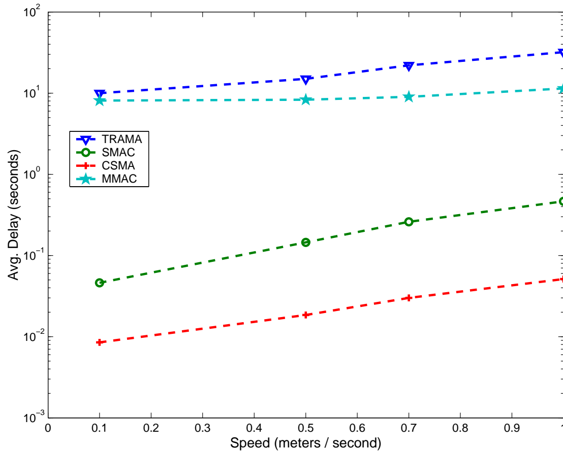
Average Packet Delay (increasing Mobility)
