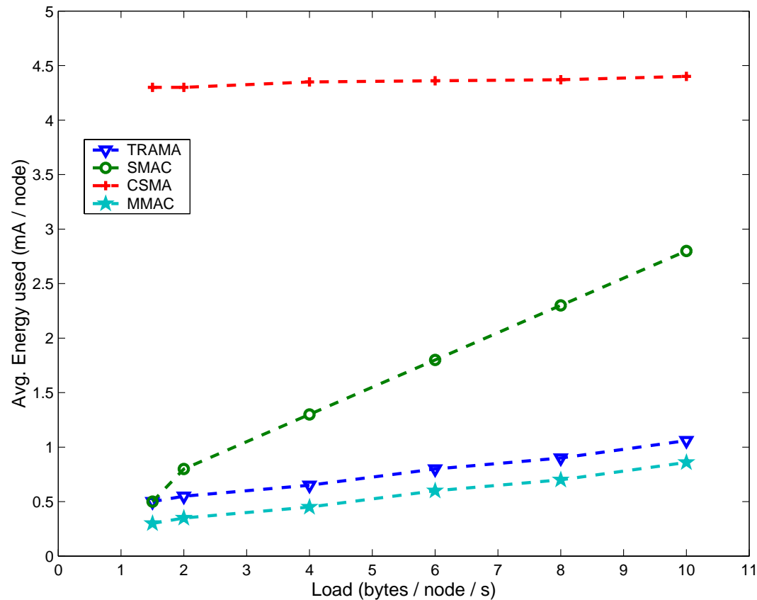
Average Energy consumed per Node (Variable Traffic)
